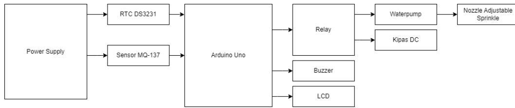
Fig 1. Block Diagram
